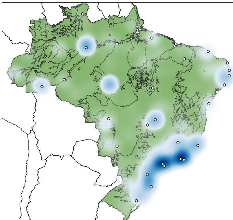
Figure 2. Heat map of anuran observations in Brazil in iNaturalist (n = 8190). Darker blue shades represent a higher density of observations concentrated around major cities.
