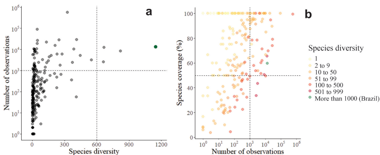
Figure 1. (a) Relation between species diversity (total number of species based on AmphibiaWeb) and the number of observations on iNaturalist. Each circle represents a country and darker circles indicate that the number of observations and species diversity among multiple countries fall to the same location. The green filled dot in the upper right quadrat represents Brazil. (b) Relation between the number of observations and species coverage on iNaturalist. The color of the circles indicates a gradient of species diversity with the green dot in the upper right quadrat indicating Brazil with over 1000 amphibian species. Note that for both graphs the axes with number of observations are on a logarithmic scale.
