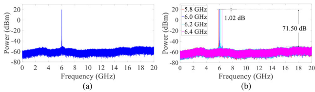
Fig. 4 Electrical spectrums at the output of the frequency divider for (a) an 18 GHz microwave signal and (b) different frequency microwave signals into the frequency divider
