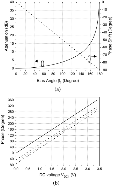
Fig. 2. (a) Output RF signal attenuation (solid line) as a function of the bias angle \beta_3 for \beta_1=0 , and the corresponding output RF signal phase shift (dashed line). (b) Output RF signal phase shift versus the DC voltage V_{DC1} into the DDMZM RF port for V_{\pi,RF}=1.7 V when the bias angle \beta_3 is set to obtain 0 dB (solid), 3 dB (dashed), 6 dB (dotted) and 10 dB (dashed-dotted) output RF signal attenuation.
