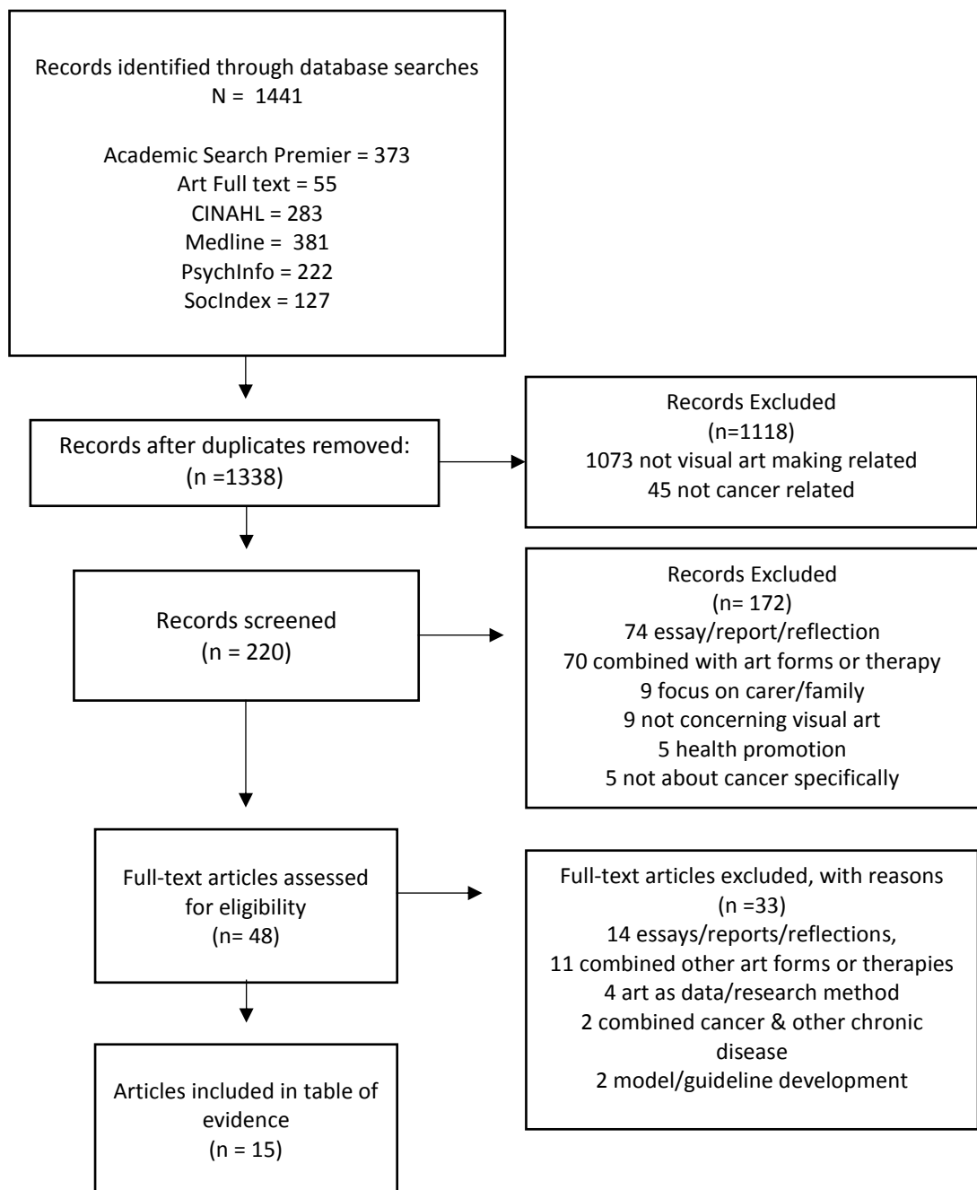
Figure 1. Search Strategy
