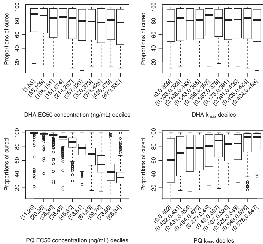
Figure 4 Distribution of proportions cured within the EC 50 and k 1 deciles derived from the 5000 parameter sets for the anti-malarial combination therapy, dihydroartemisinin (DHA) and piperavaquin (PQ). Top panels are for dihydroartemisinin (EC 50 – left hand side, k max right hand side) and bottom panels are for piperavaquin (EC 50 – left hand side, k max right hand side).
